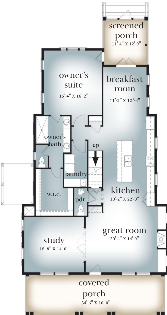
First Floor
